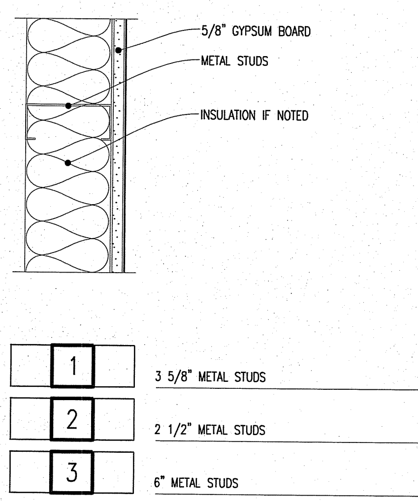
PARTITION NO SCALE C1010FP-21
