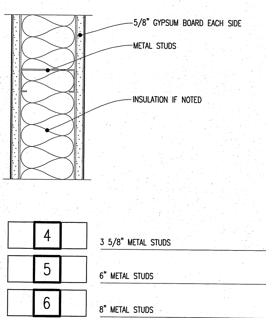
PARTITION NO SCALE C1010FP-22
