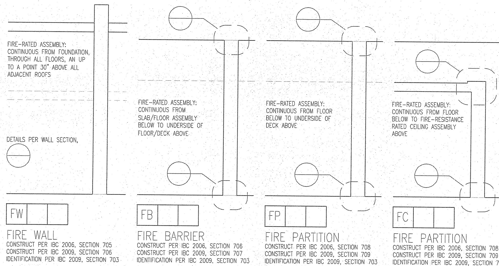
E1 PARTITION CONFIGURATIONS NO SCALE
