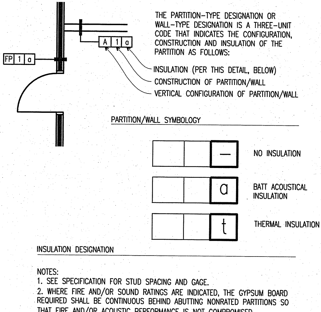
C1 PARTITION-TYPE LEGEND NO SCALE C1010FP-01
