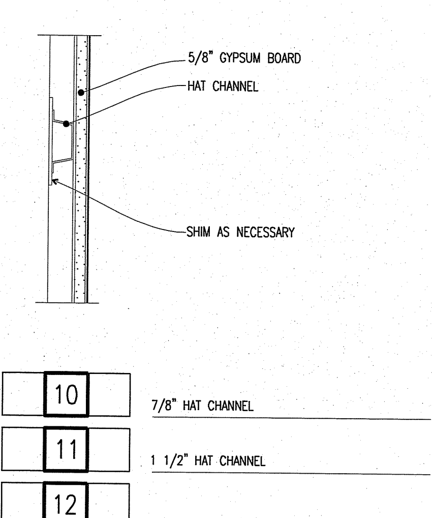
FURRING NO SCALE C1010FP-76
